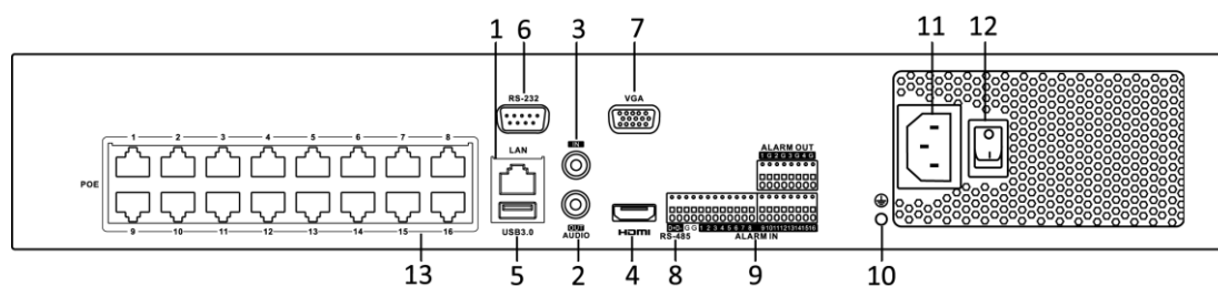
Figure 1. 9 DS-7700NI-E4/P-serie
